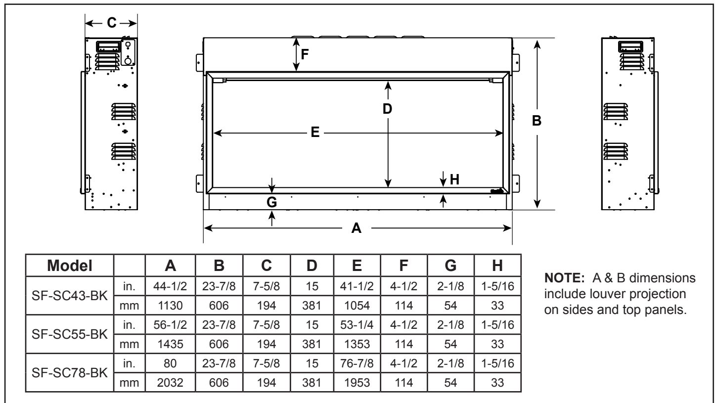
Figure 3.1 Appliance Dimensions
