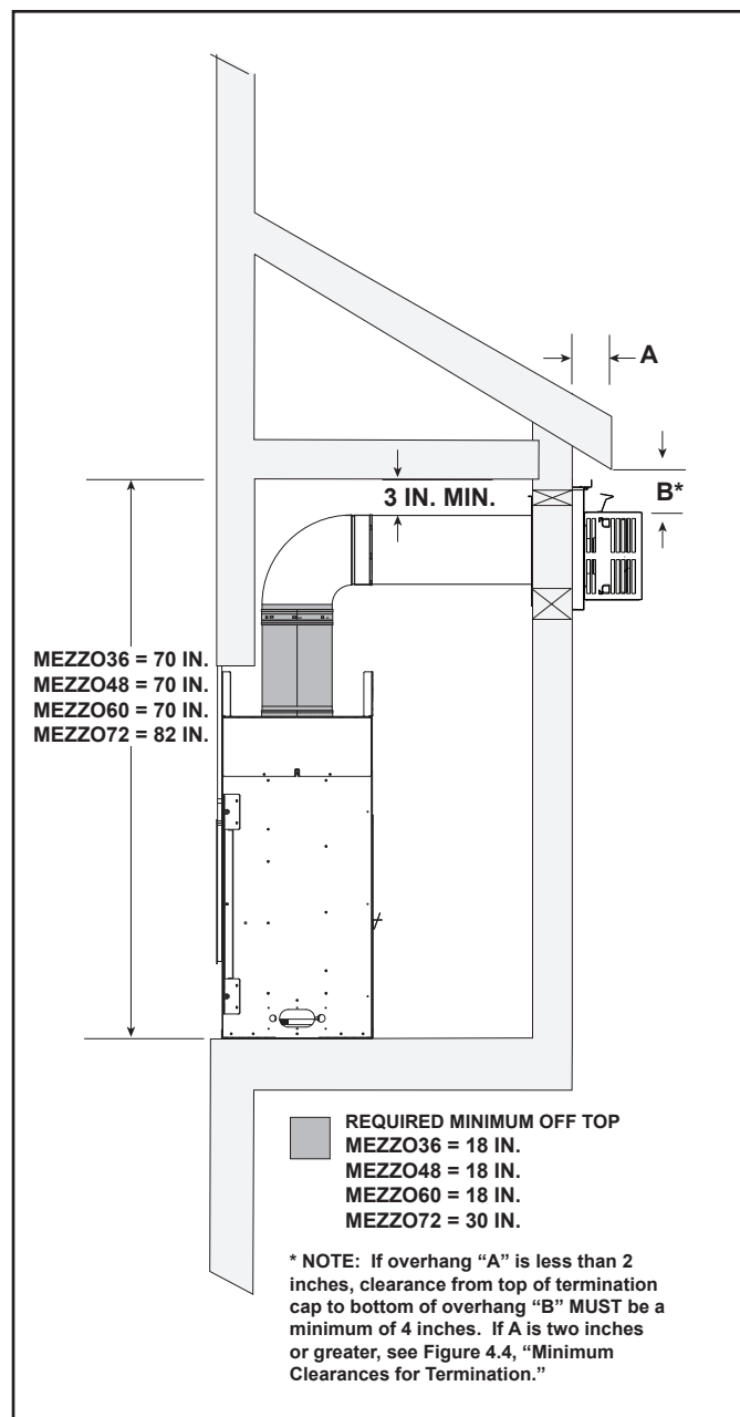
Figure 3.19 Exterior Chase - Minimum Height Requirements
