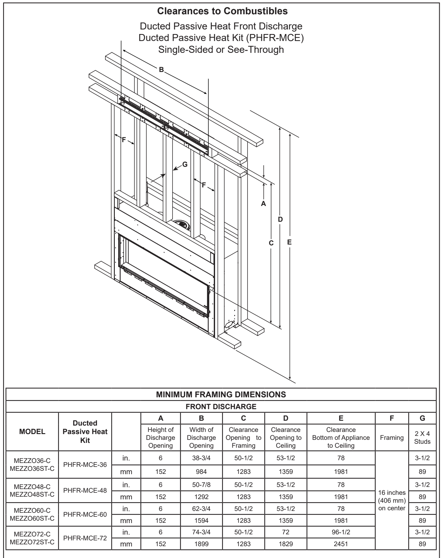
➔ Figure 3.17 Clearances to Combustibles - Ducted Passive Heat Front Discharge
