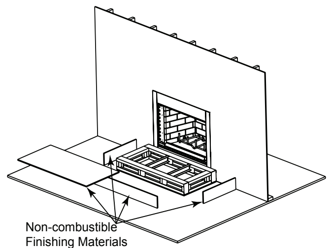
Figure 7.7 Raised Platform Hearth Extension-Finishing
