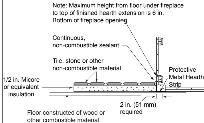
Figure 7.4 Hearth Extension Construction
