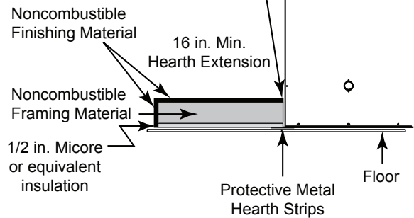
Figure 7.5 Raised Platform Hearth Extension Detail
