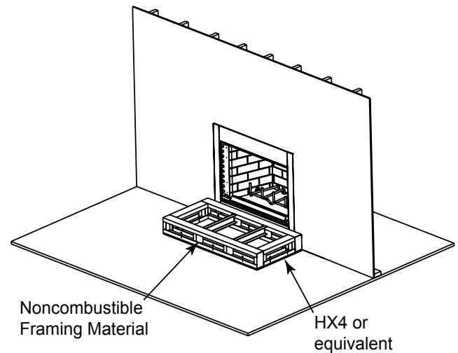
Figure 7.6 Raised Platform Hearth Extension-Framing
