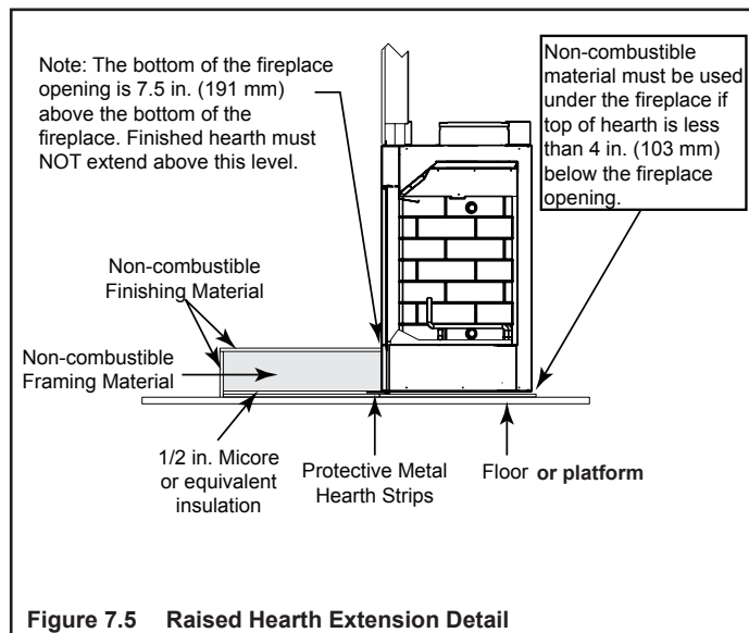
Figure 7.5 Raised Hearth Extension Detail
