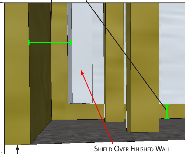
COMBUSTIBLE WALL Figure 41
