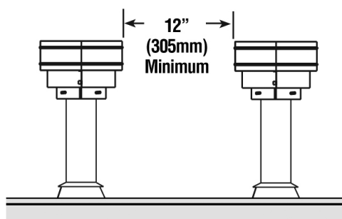
Figure 37: Multiple Termination Clearance
