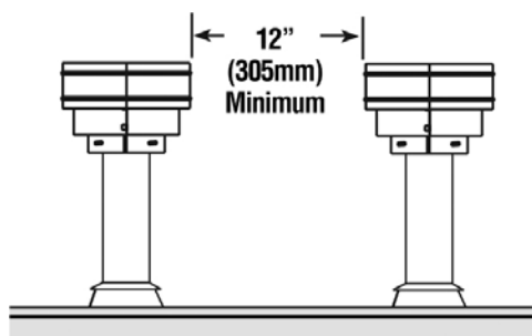
Figure 40: Multiple Termination Clearance
