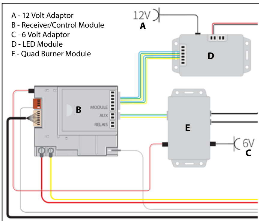
Figure 4: AC Adapter Connection
