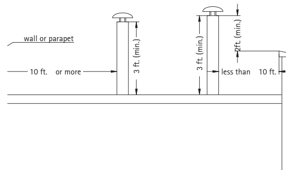
flat roof
