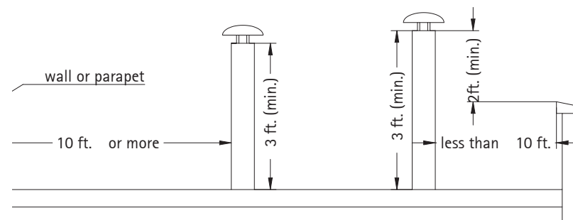
flat roof
