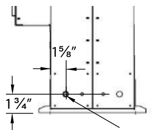
1/2" MPT gas
