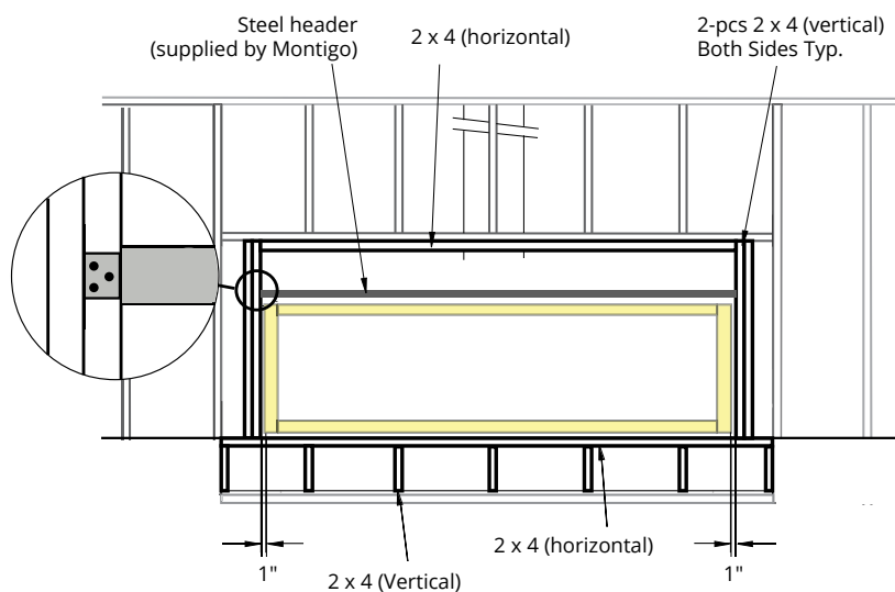
Figure 3.i Recessed Fireplace installation
