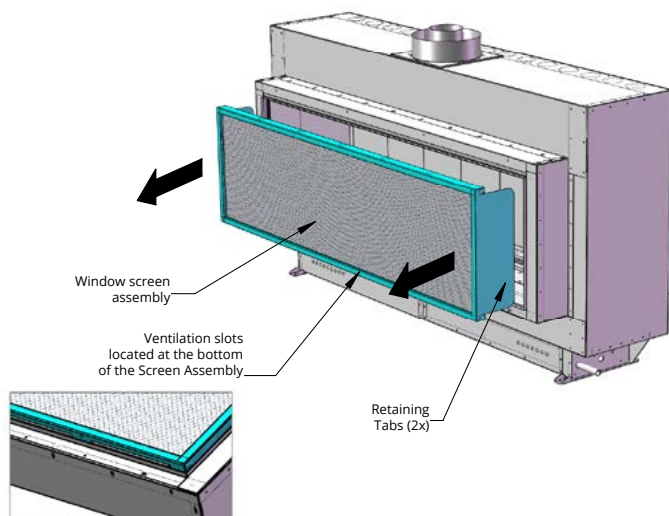
Figure 11. Screen Removal.
