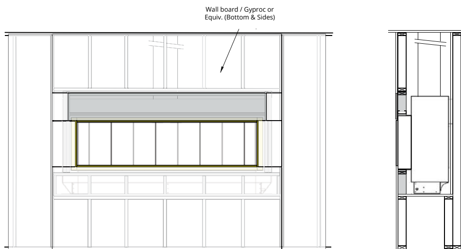
Figure 10.b Fireplace installation (Cut the remainder of Gyproc / Wall board to complete the fireplace surround).
