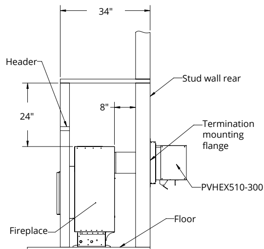
Figure 3.b Clearances for straight rear vented installation with PVHEX58-300.
