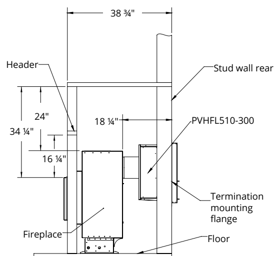
Figure 3.c Clearances for straight rear vented installation with PVHFL510-300.
