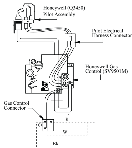
Figure 14. Gas valve
