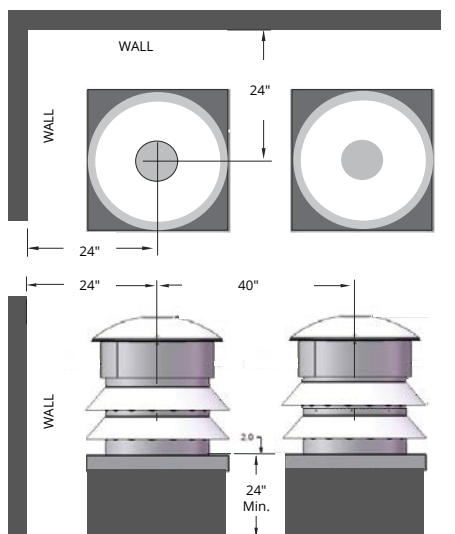
Figure 15.b PVVEX510-300 clearances
