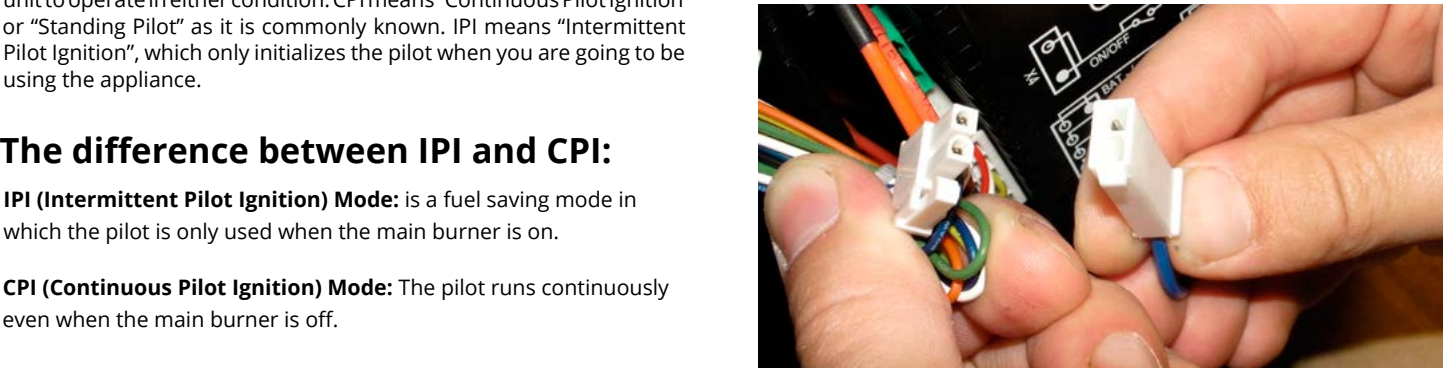
Figure 6.1 Locate Jumper cable
