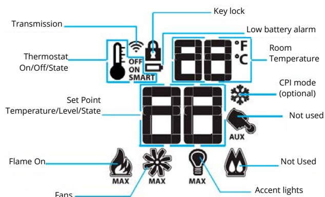
Figure 9.10 Remote Control LCD Display
