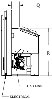
Figure 1.4 Unit dimensions (Tolerance ± ⅛") [1.25 mm]
