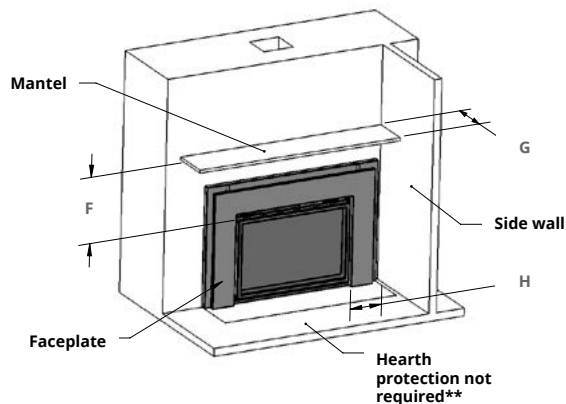
Figure 2.1 Install clearances
