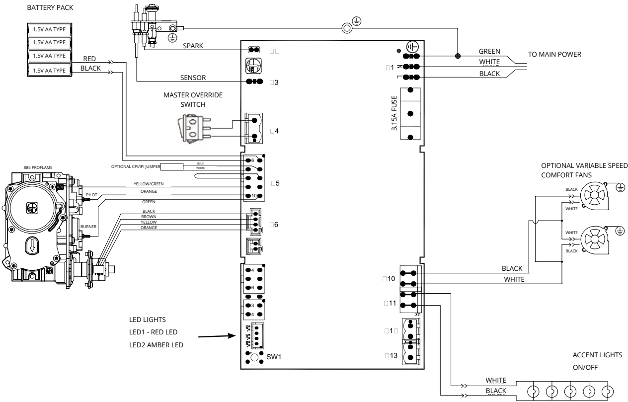
Figure 9.7 SIT Proflame 2 Electronic Ignition
