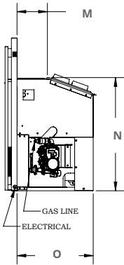
Figure 1.3 Unit dimensions (Tolerance ± ⅛") [1.25 mm]
