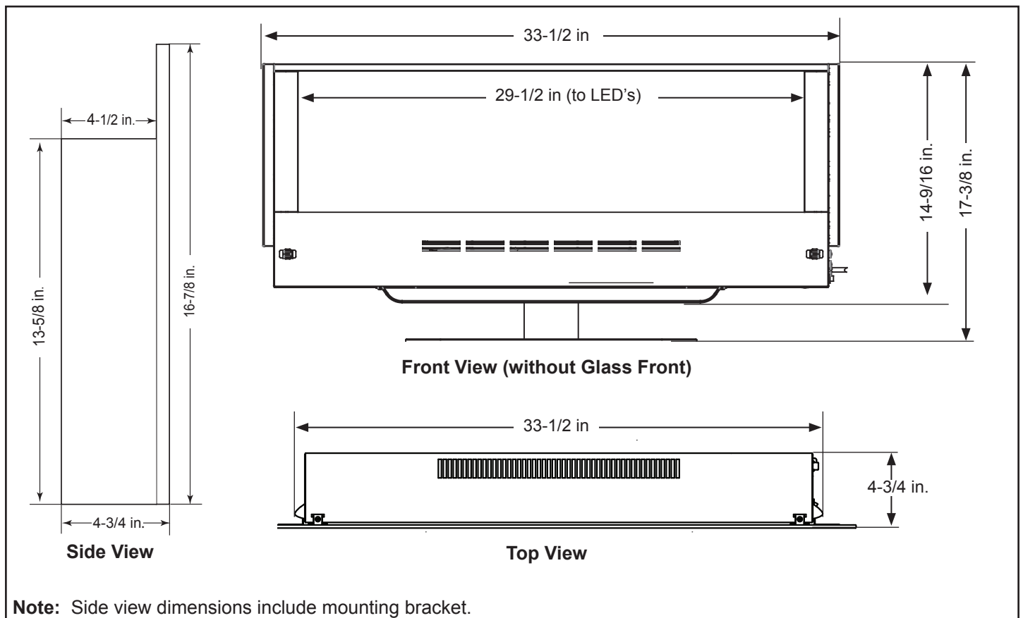
Figure 3.1 Appliance Dimensions
